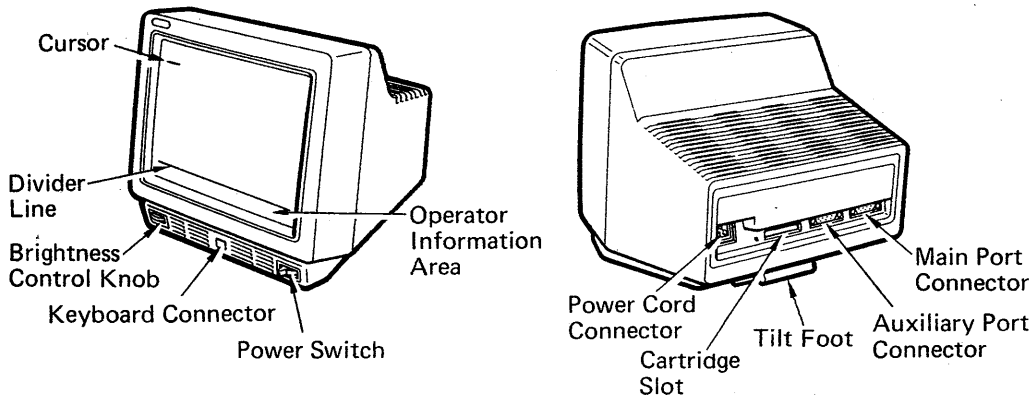
Figure 1-3. Video Element
