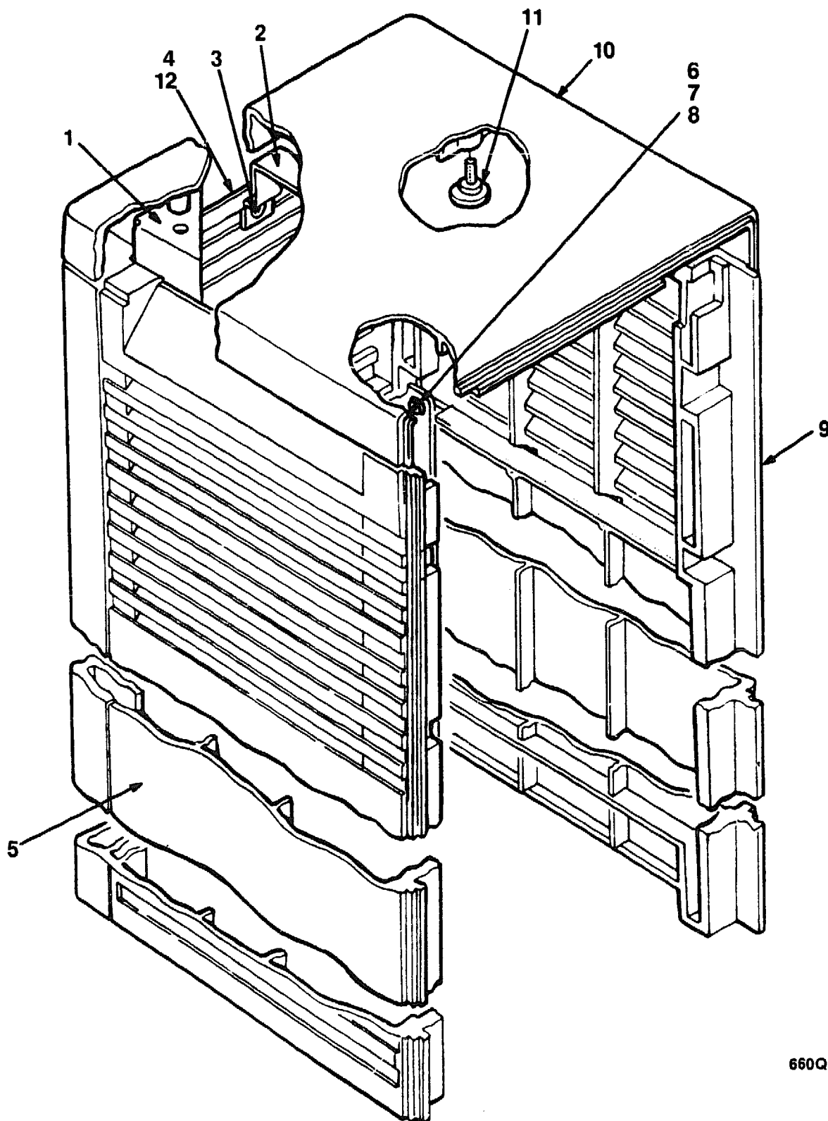
Figure 5. Enclosure Assembly, Shell
