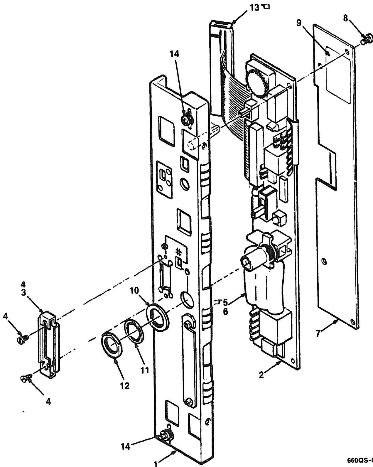
Figure 2. Bulkhead Assembly, H3602 Module
