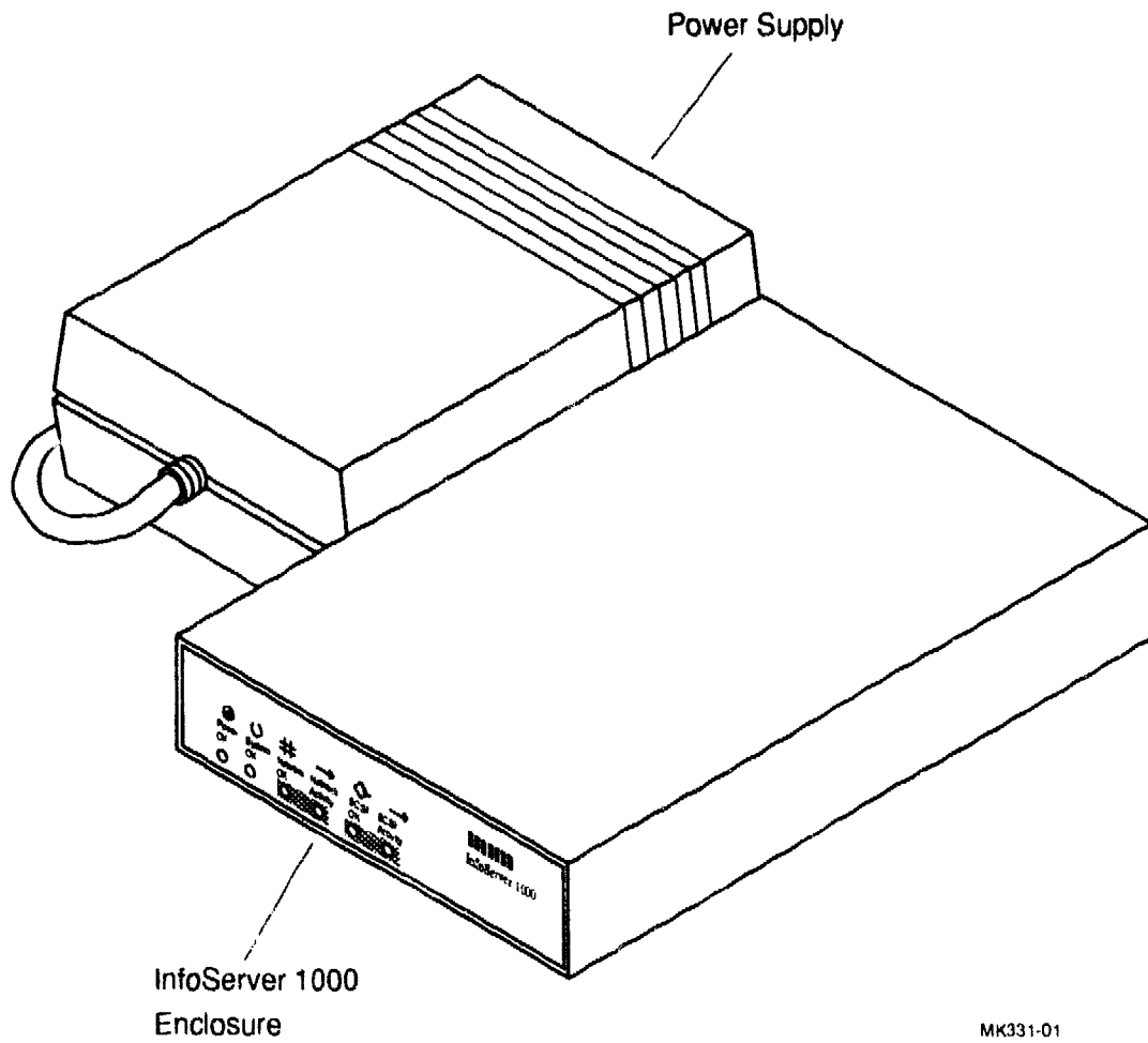
Figure 1-1 Standalone InfoServer 1000
