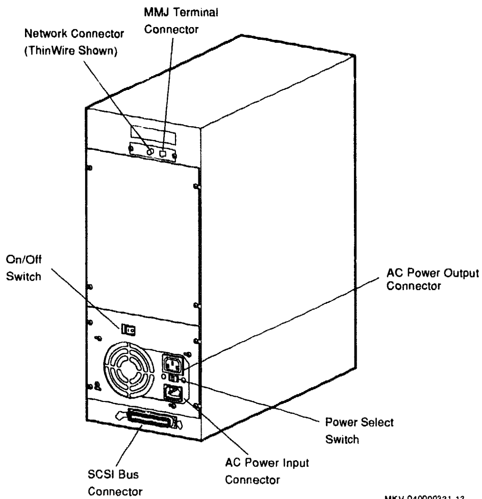
Figure 3-3 InfoTower Ports and Connectors
