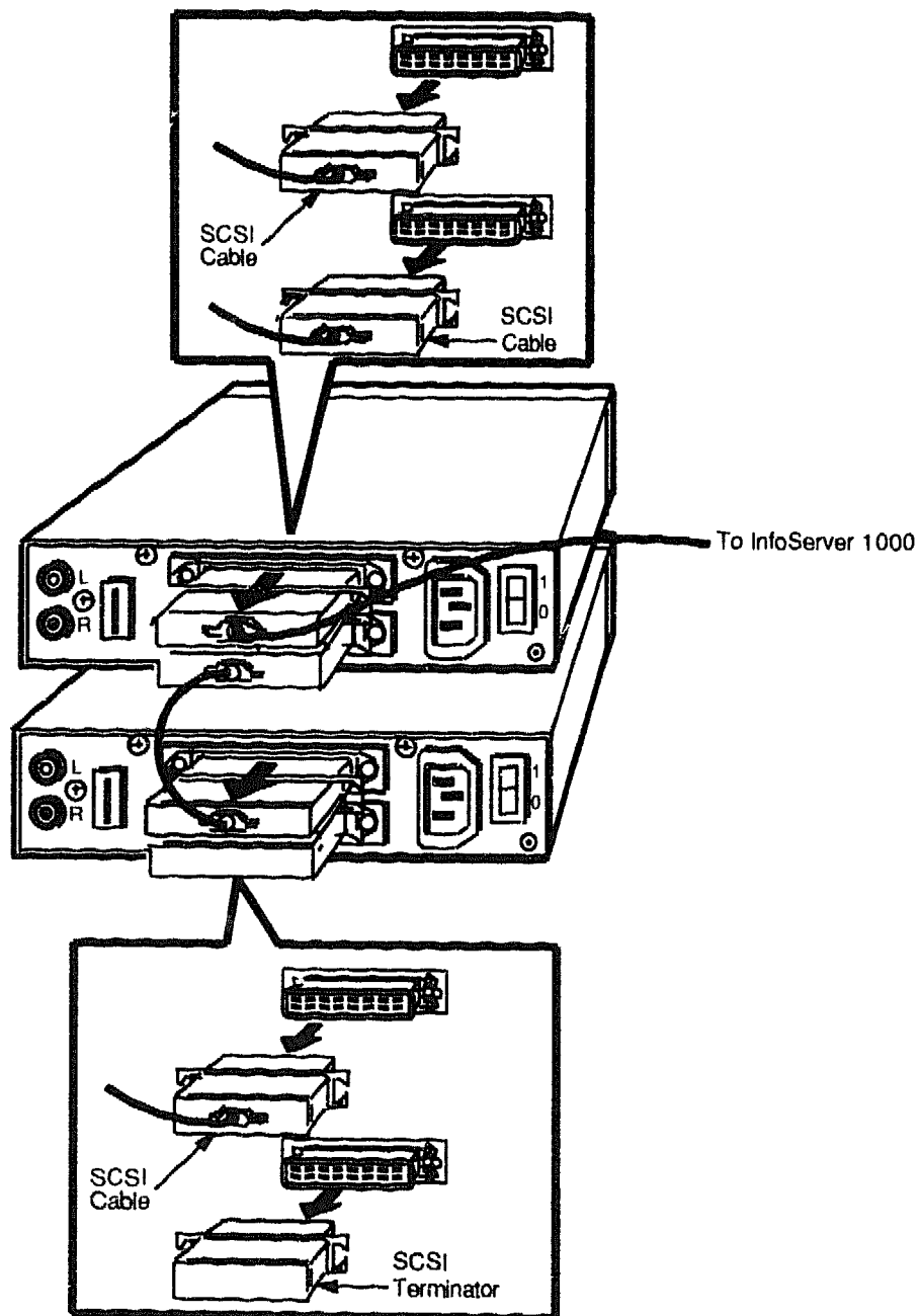
Figure 5-2 Connecting Two RRD42 Expansion Peripherals
