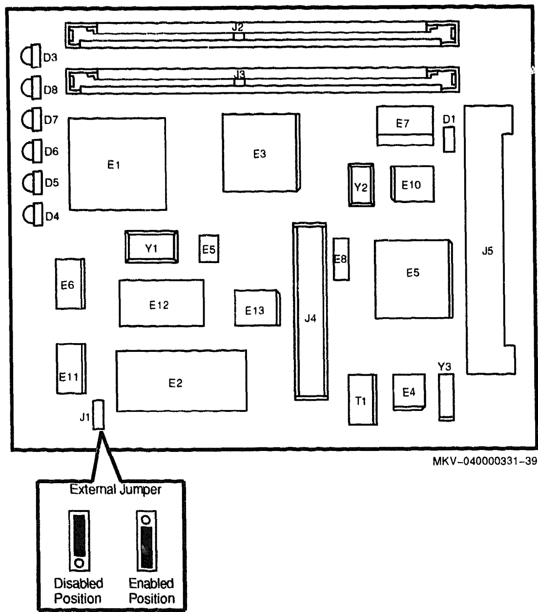
Figure 7-1 Setting the External Jumper (J1)
