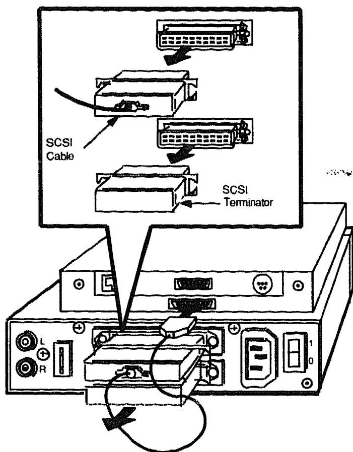
Figure 5-1 Connecting One RRD42 Expansion Peripheral
