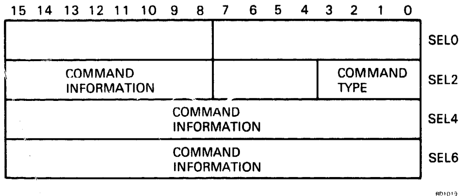
Figure A-3 CSR Command Format
