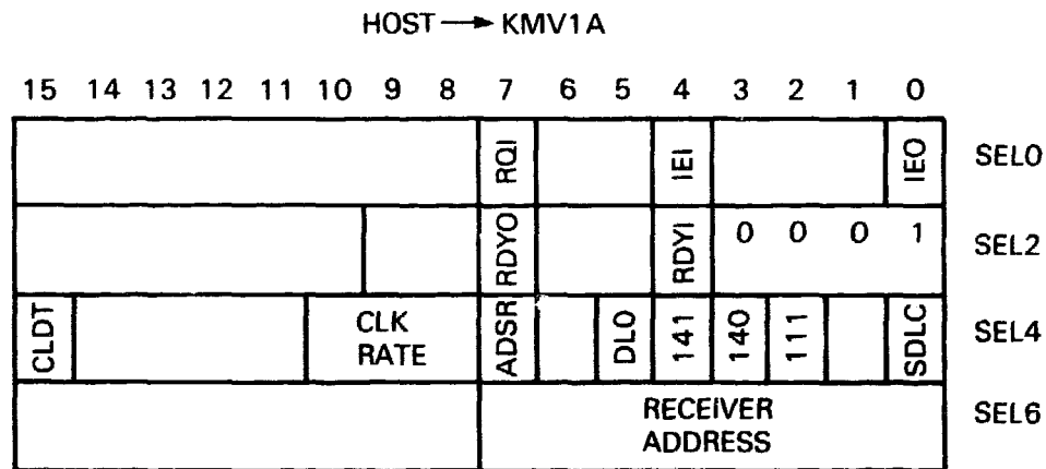
Figure A-12 Configure Command
