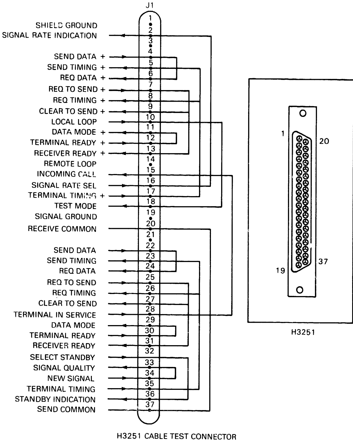
Figure 5-4 K MV1A Loopback Connector H3251
