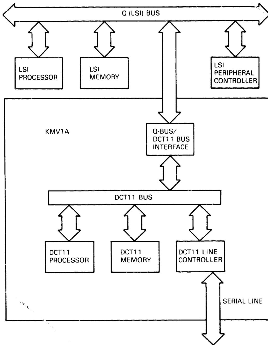
Figure 4-1 KMV1A Architecture
