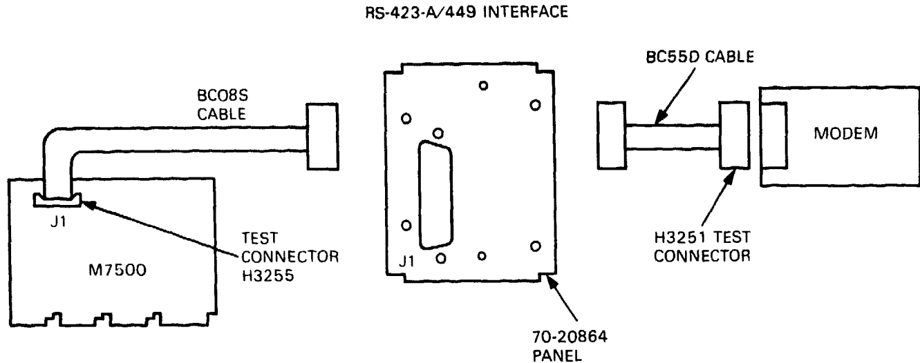
Figure E-1 General Cabinet Kit Diagram
