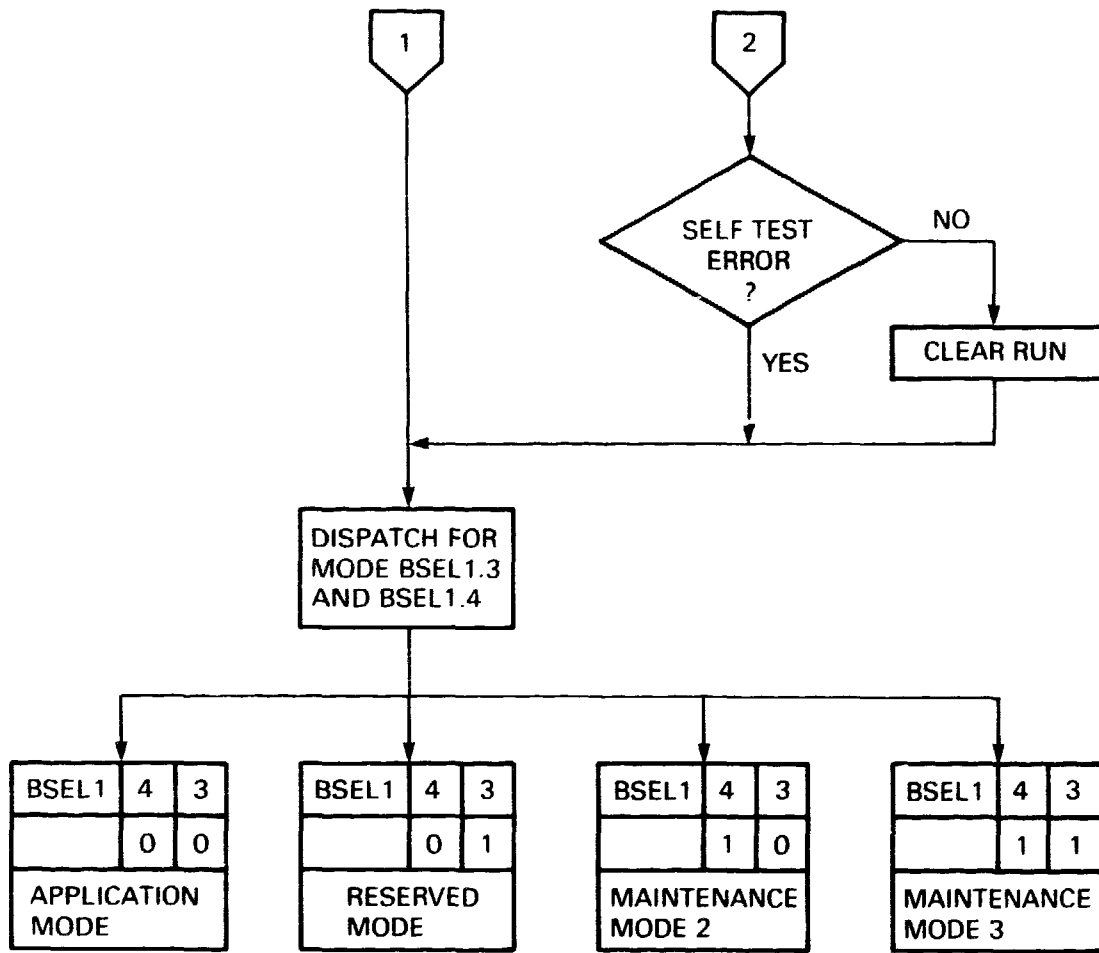
Figure 3-3 Initialization and Mode-Setting Flowchart (Cont.)
