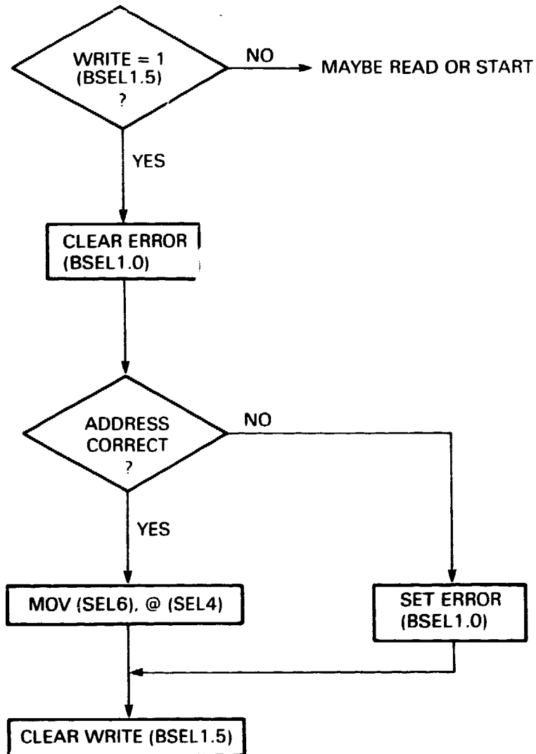
Figure 3-4 Write into RAM Flowchart
