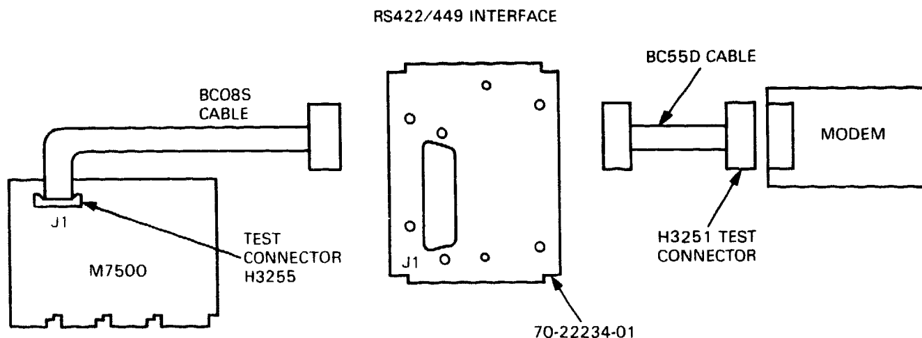
Figure D-1 General Cabinet Kit Diagram
