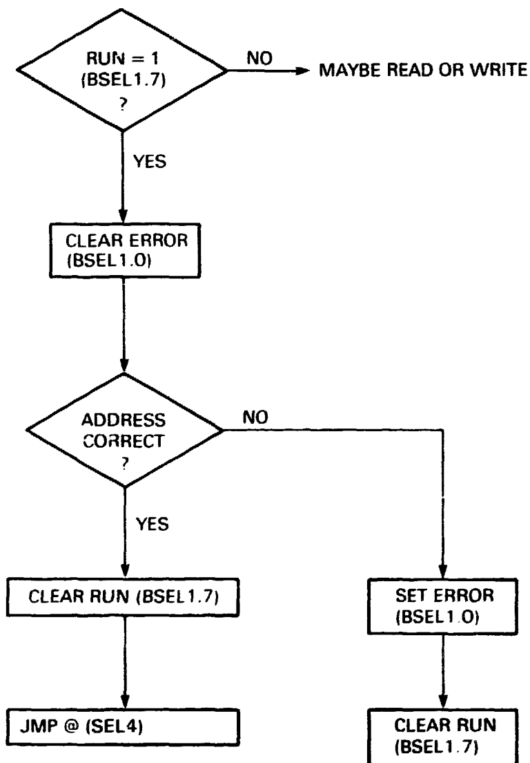
Figure 3-6 Run Flowchart
