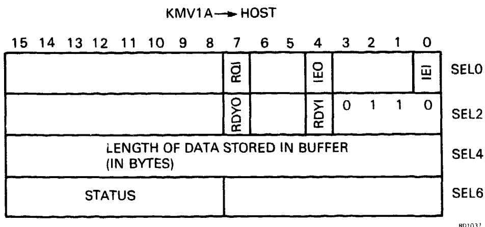
Figure A-21 Reception Buffer Response
