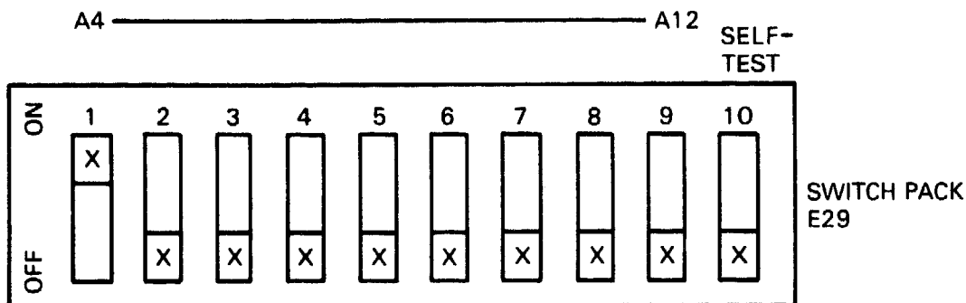
Figure 2-2 Address Switch Setting Example: 760020 8
