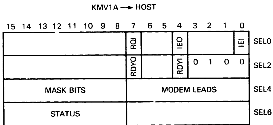
Figure A-16 Modem Change Response
