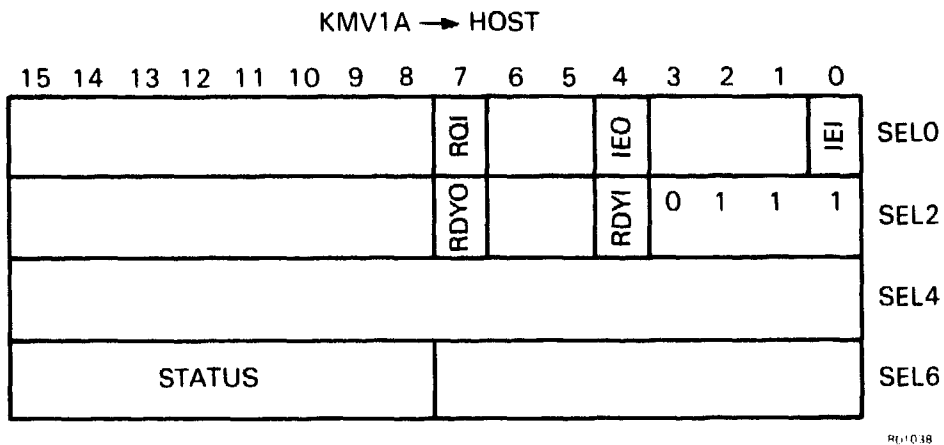
Figure A-23 Transmit Abort Response
