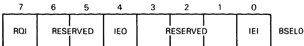
Figure A-1 Control Register BSEL0
