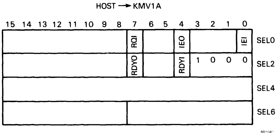
Figure A-24 Receive Abort Command
