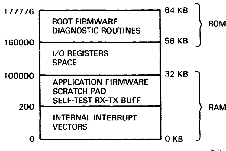
Figure 4-4 KMOV1A Memory Map
