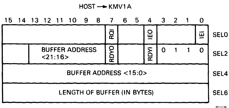
Figure A-20 Reception Buffer Command
