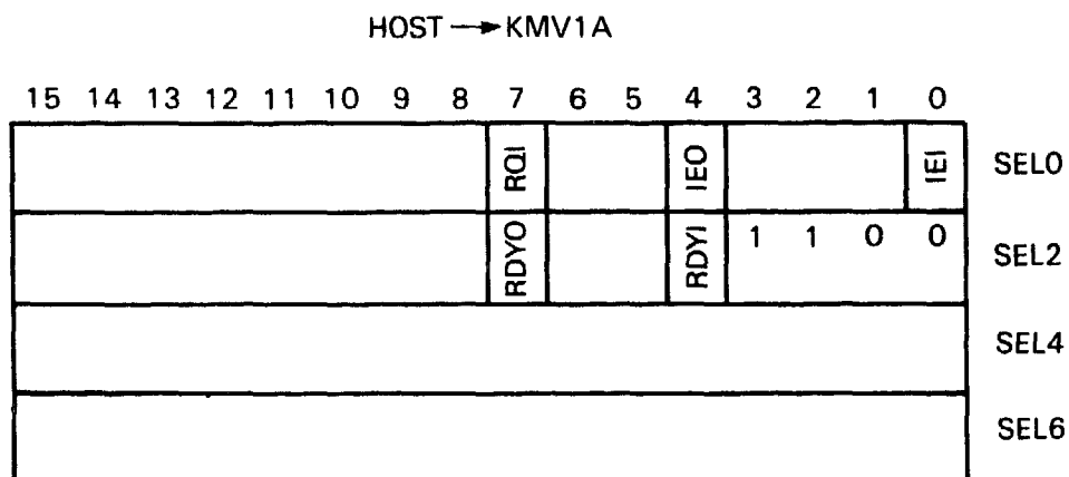
Figure A-26 Read Modem Command
