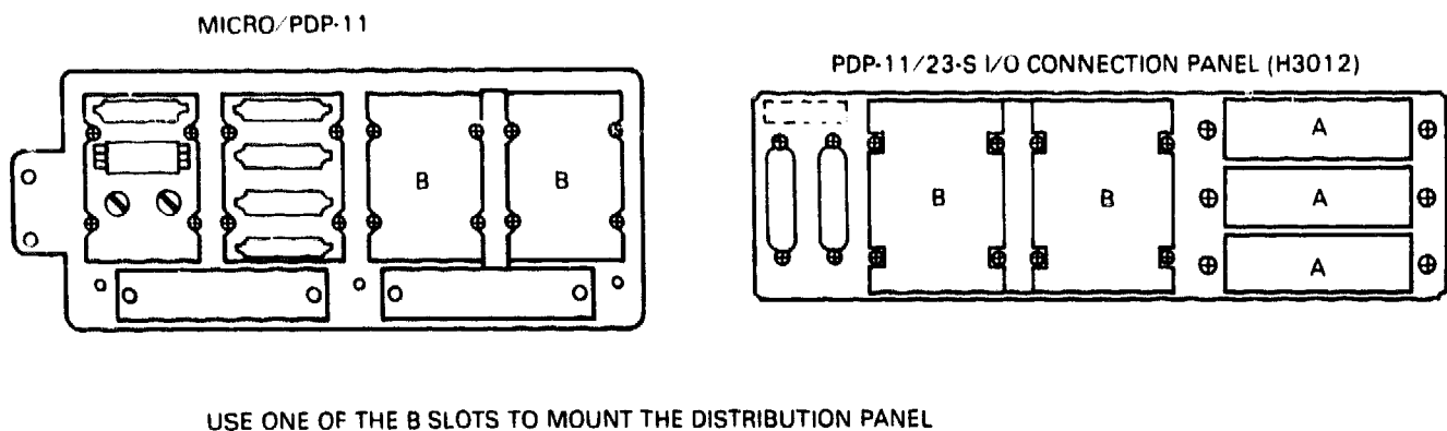
Figure D-2 Distribution Panel Installation
