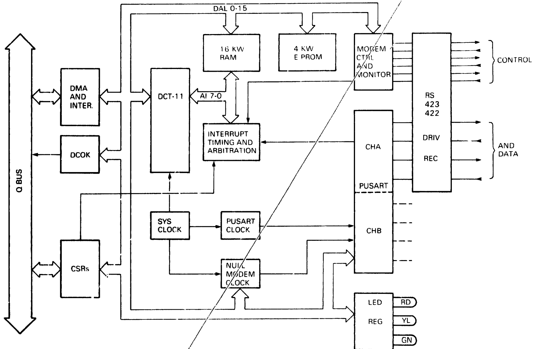
Figure 4-2 Block Diagram of the KMOV1A
