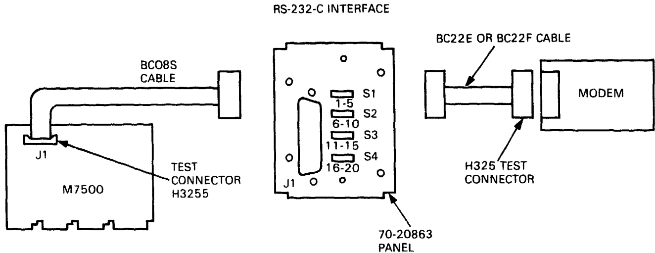
Figure C-1 General Cabinet Kit Diagram
