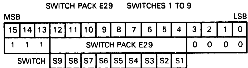
Figure 2-1 Address Switch Register Mapping
