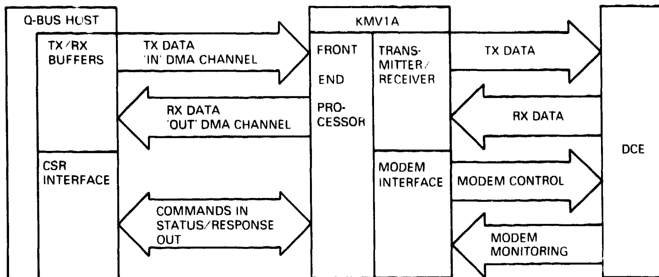
Figure 1-1 KMVIA Block Diagram
