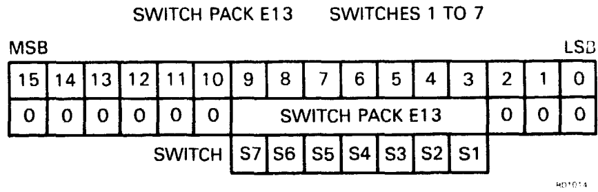
Figure 2-3 Vector Switch Register Mapping
