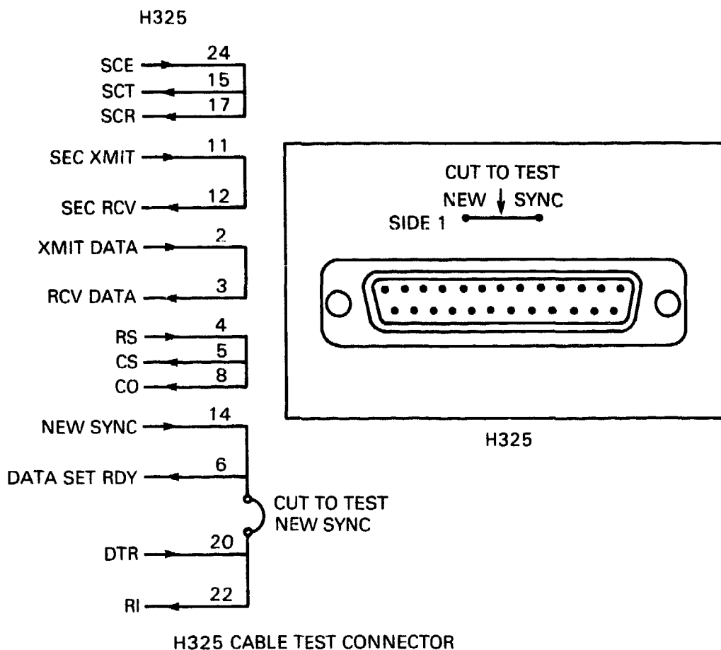
Figure 5-5 KMOVIA Turnaround Connector H325
