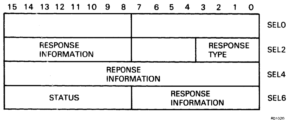
Figure A-4 CSR Response Format
