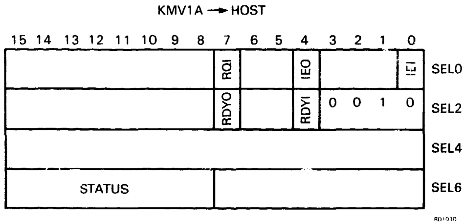
Figure A-13 Configure Response
