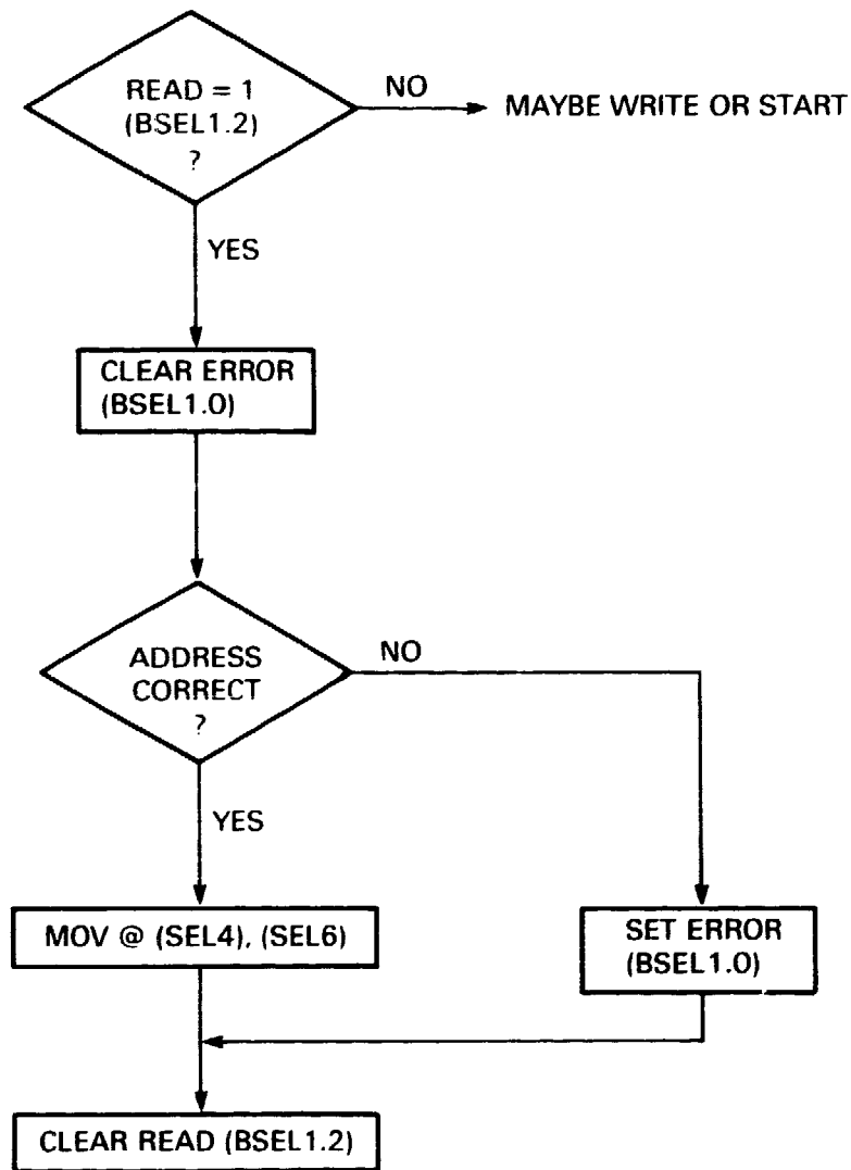
Figure 3-5 Read from RAM or ROM Flowchart
