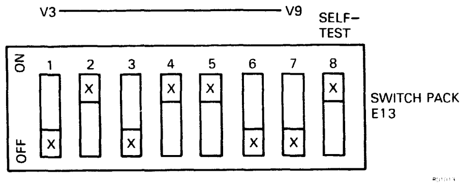
Figure 2-4 Vector Switch Setting Example: 320
