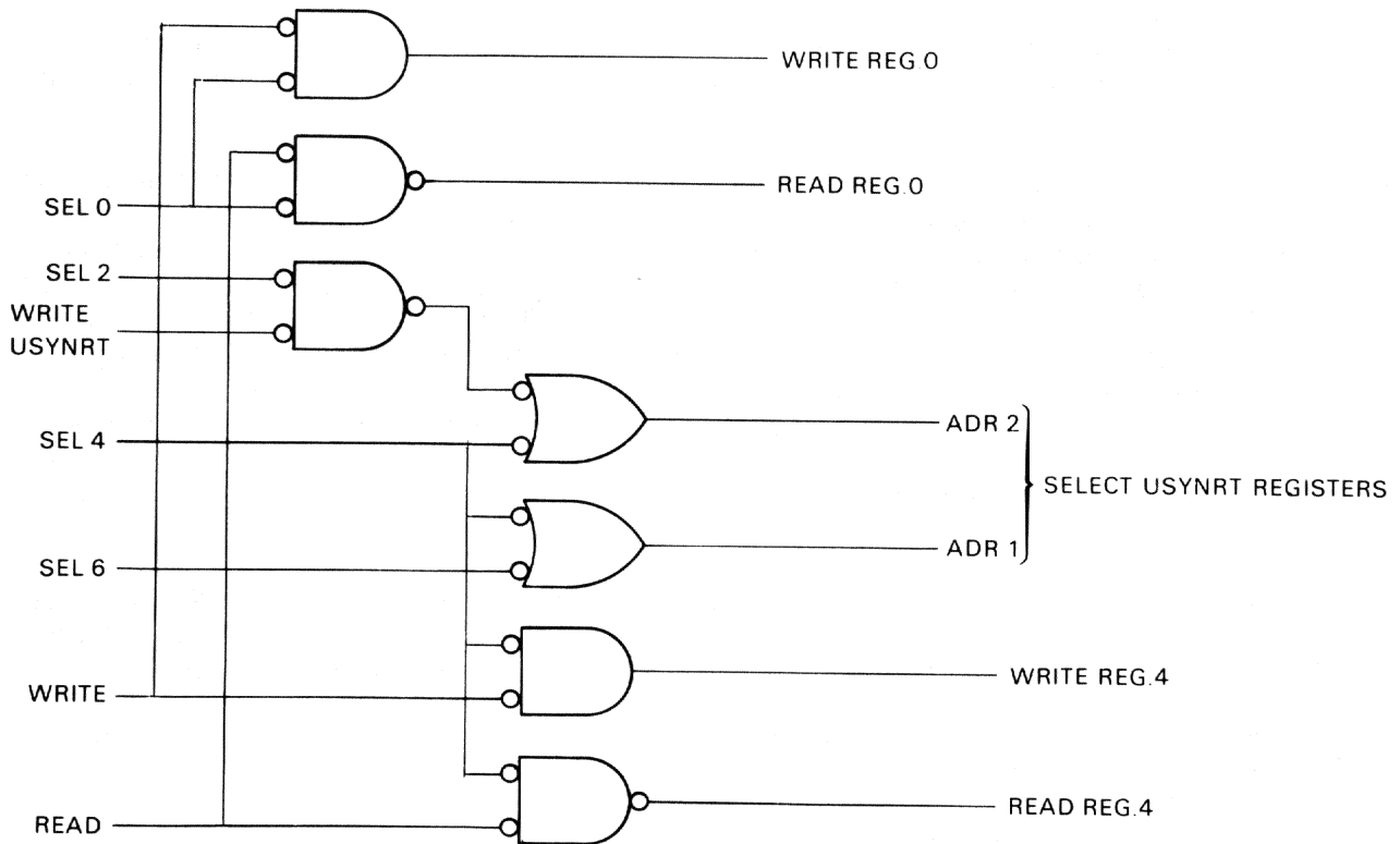
Figure 4-3 Register Decode
