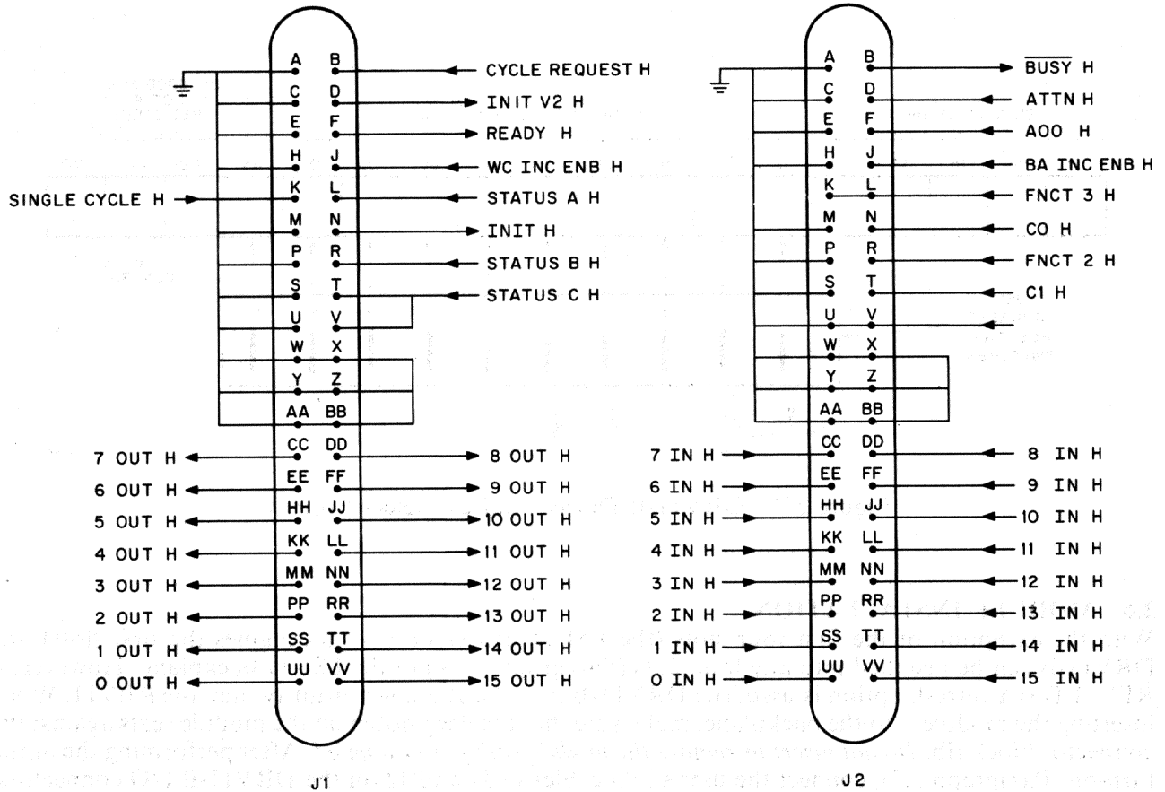
Figure 2-4 DRV11-B Connector Pin Assignments
