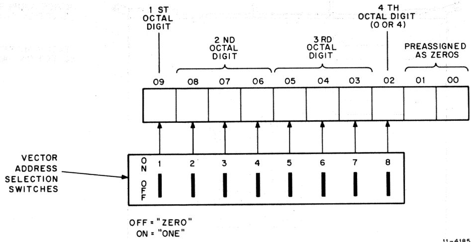
Figure 2-3 DRV11-B Interrupt Vector Address Select Format
