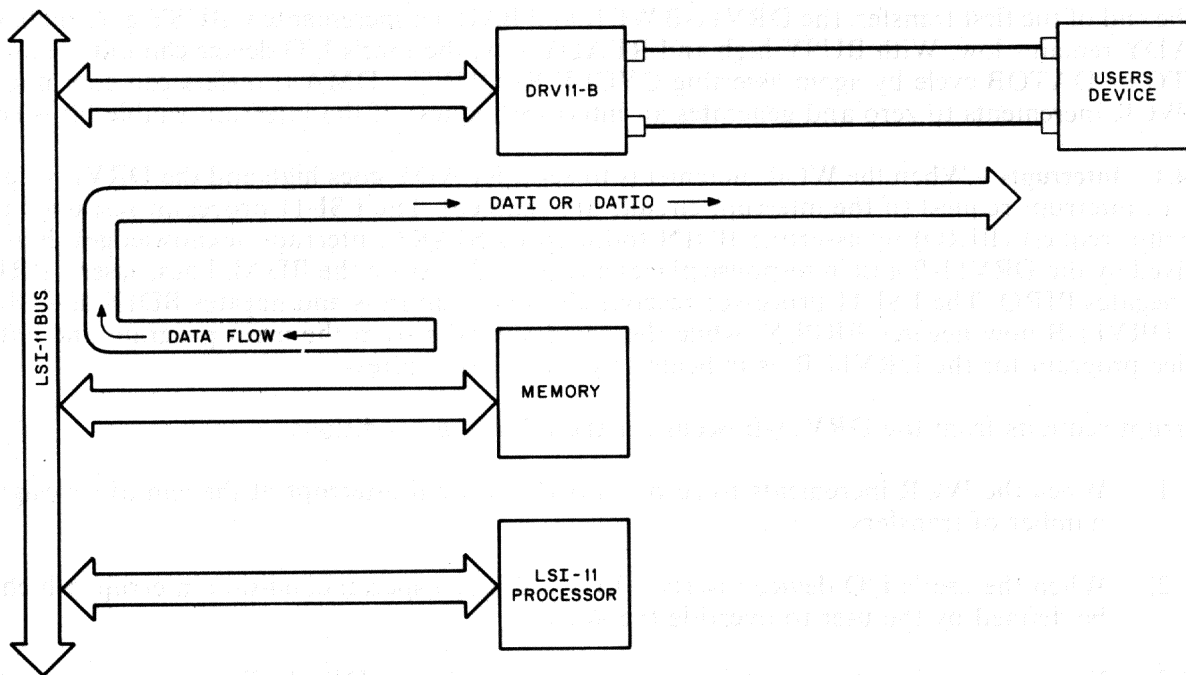
Figure 3-3 DMA DATIO/DATI Data Flow Diagram
