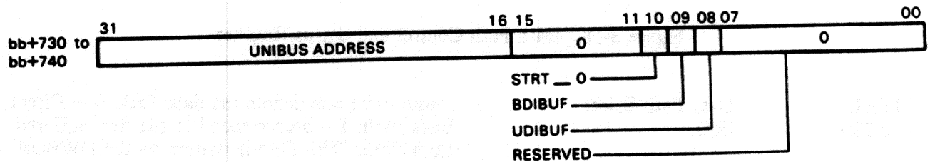
Figure 3-17 Microdiagnostic Register
