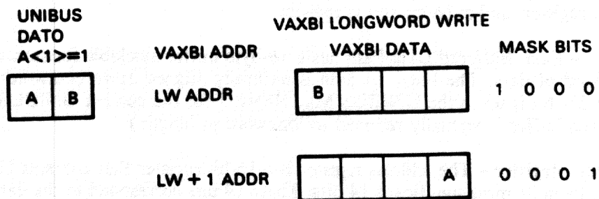
Figure I-1 DATO with UNIBUS Address Bit <01> Set
