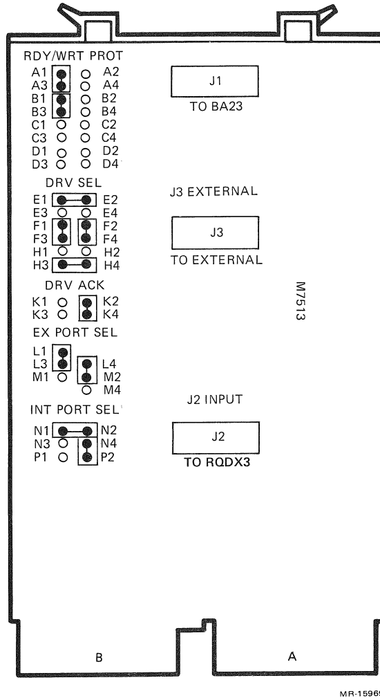
Figure 6 RQDXE Factory Jumper Configuration
