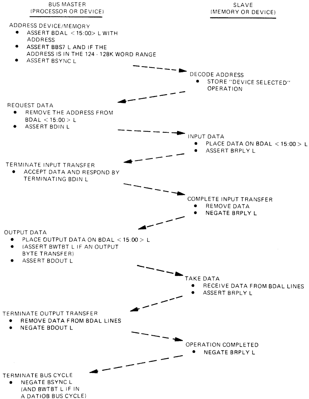
Figure 4-5 DATIO or DATIOB Bus Cycle
