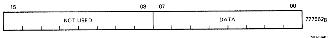
Figure 3-2 Receiver Buffer Register
