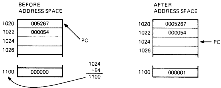
Figure 6-14 PC Relative Mode Example
