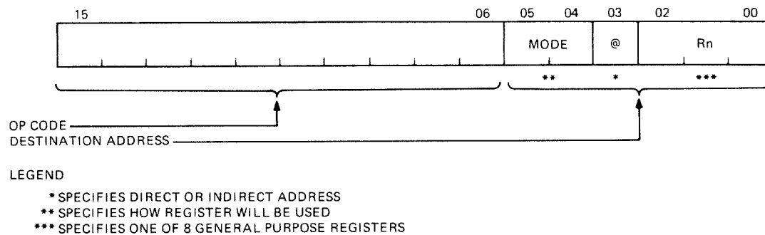
Figure 6-1 Single Operand Instruction Format
