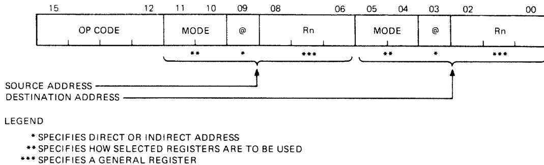
Figure 6-2 Double Operand Instruction Format
