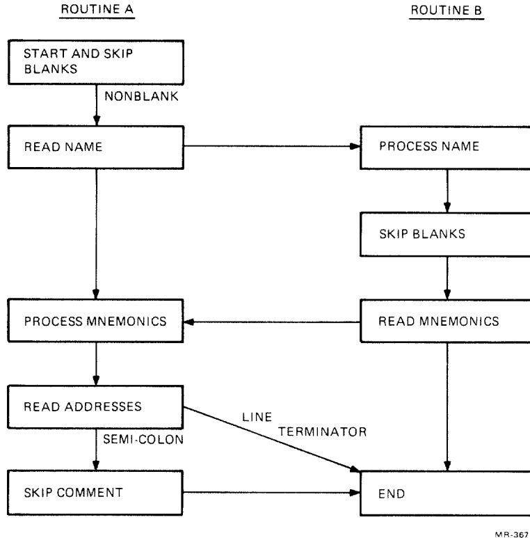
Figure 10-10 Coroutine Path
