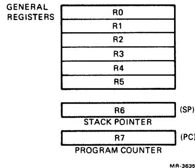
Figure 1-2 General Register
