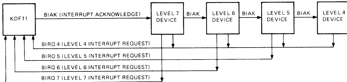
Figure 4-12 Position-Dependent Configuration
