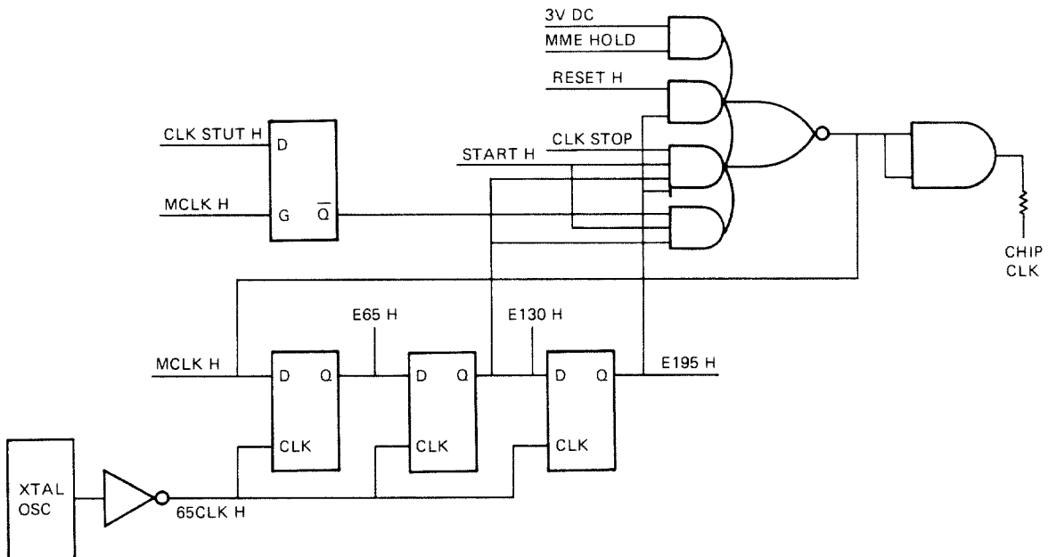
Figure 5-6 Clock Generator
