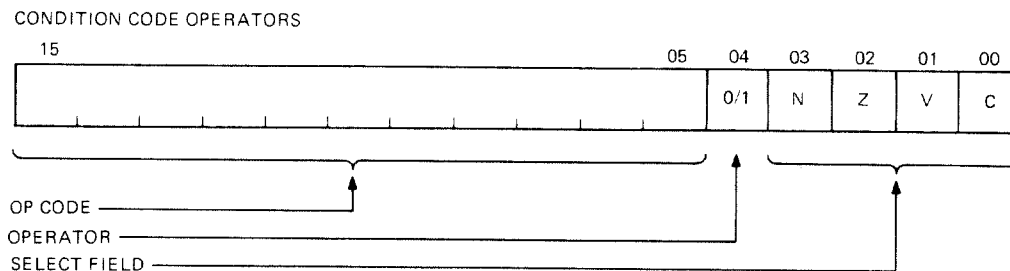
Figure 7-6 Condition Code Operators Format
