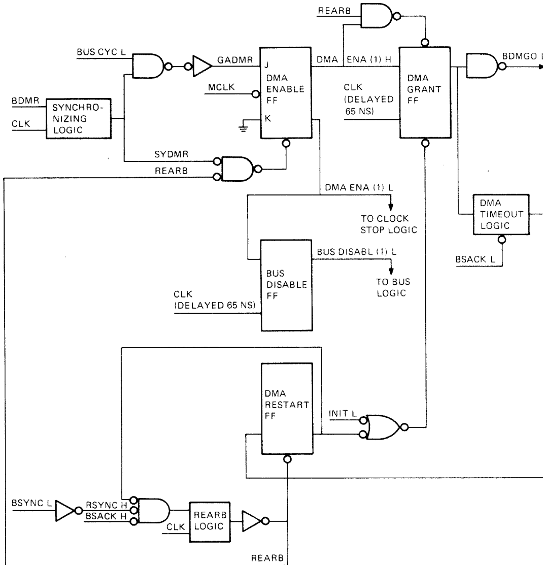
Figure 5-5 DMA Logic
