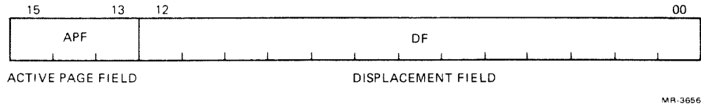
Figure 8-8 Interpretation of a Virtual Address
