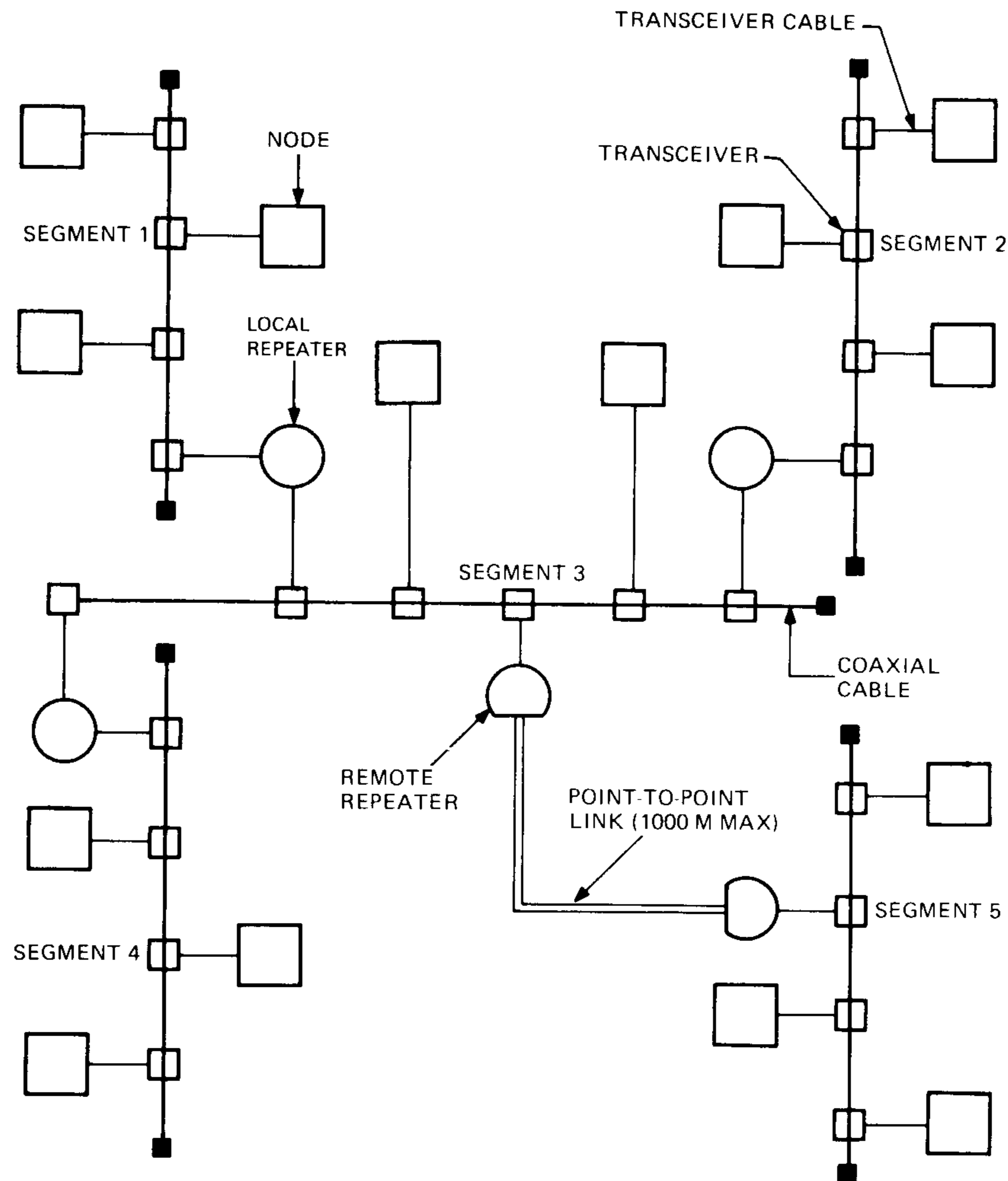
Figure 1-1 Large-Scale ETHERNET Configuration
