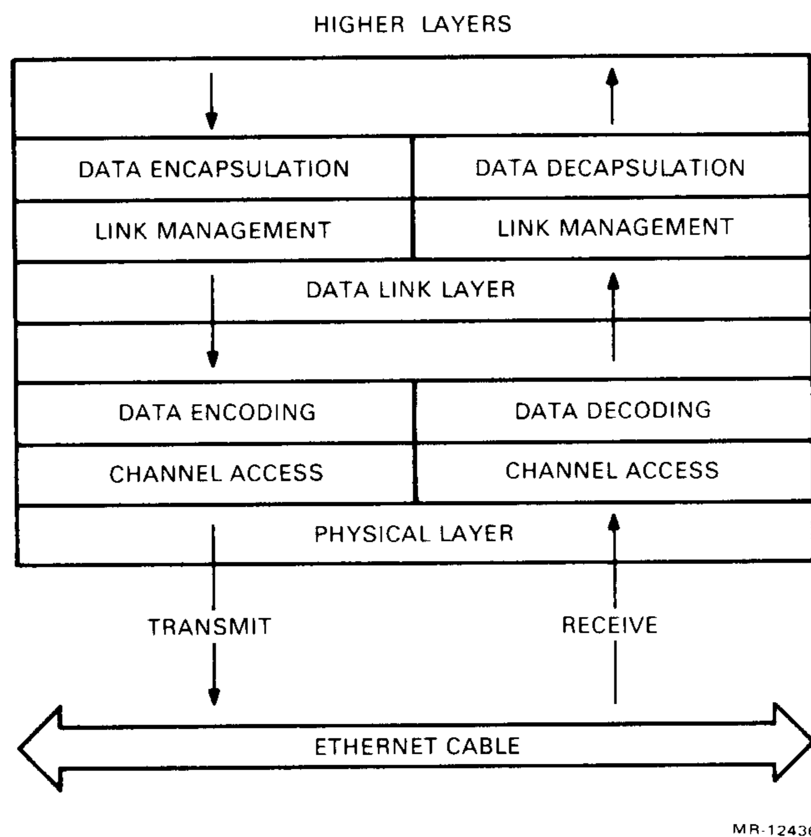
Figure 1-2 ETHERNET Layer Functions
