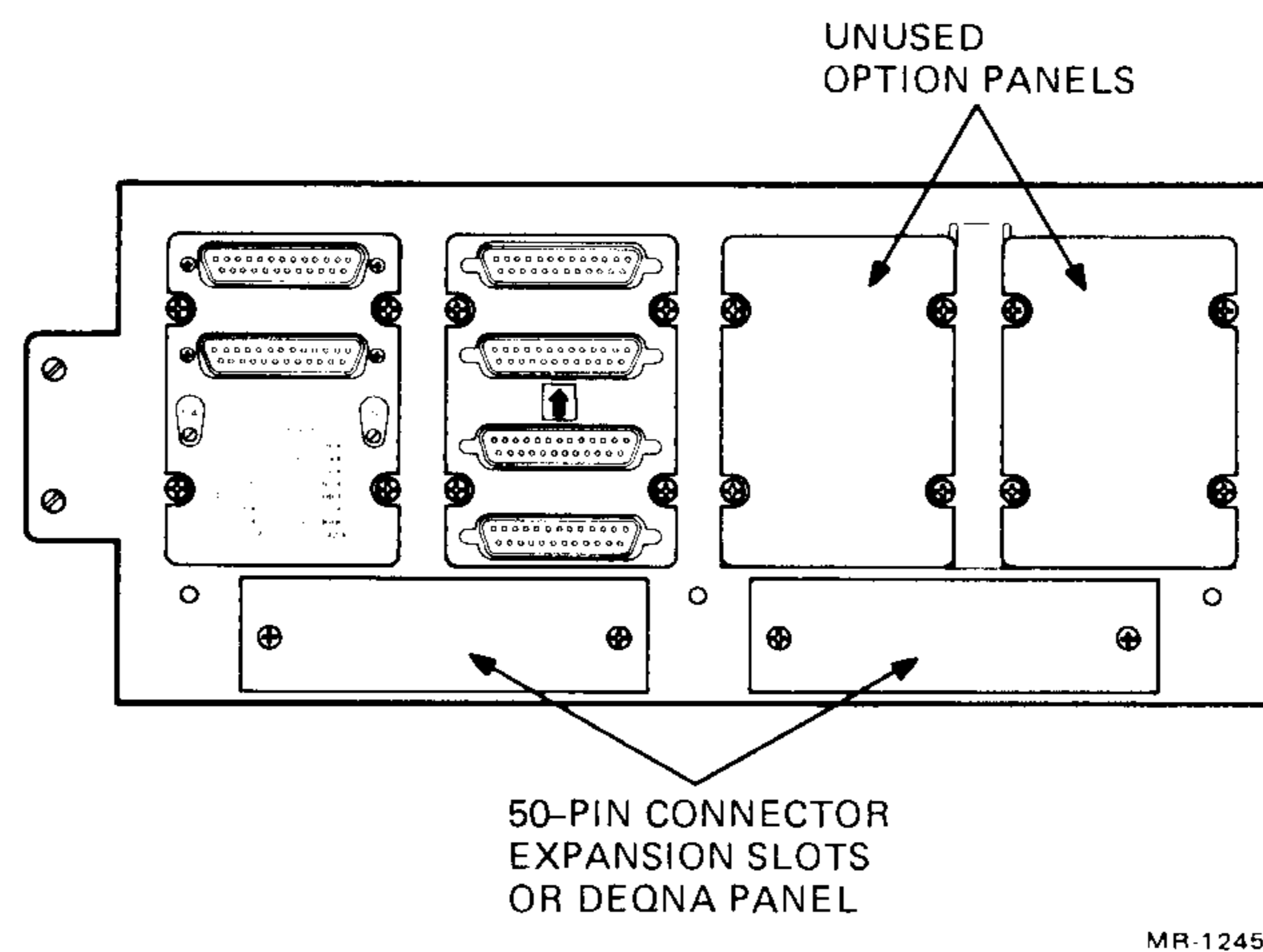
Figure 2-1 Patch and Filter Panel Assembly
