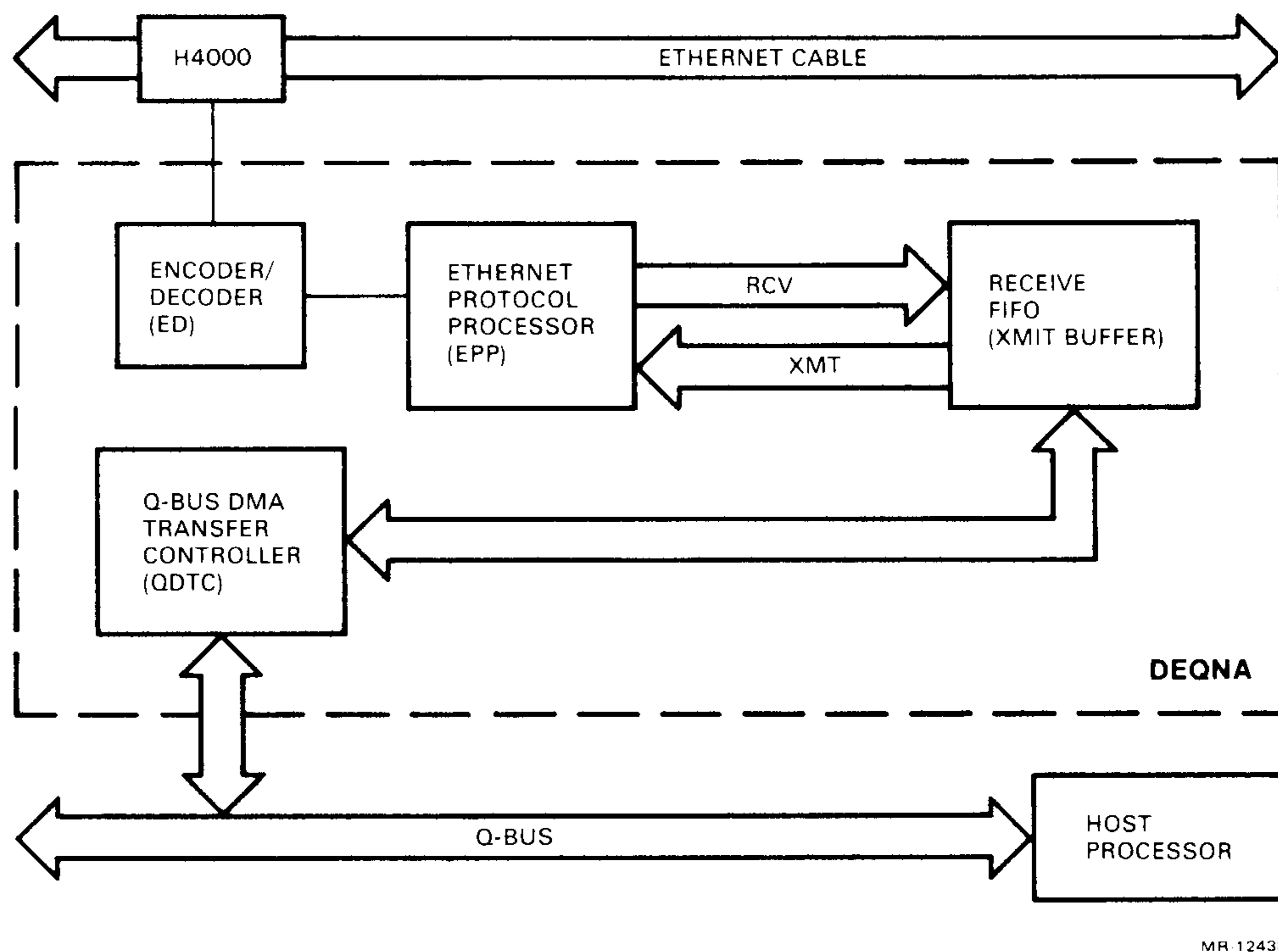
Figure 1-5 DEQNA Major Functional Areas
