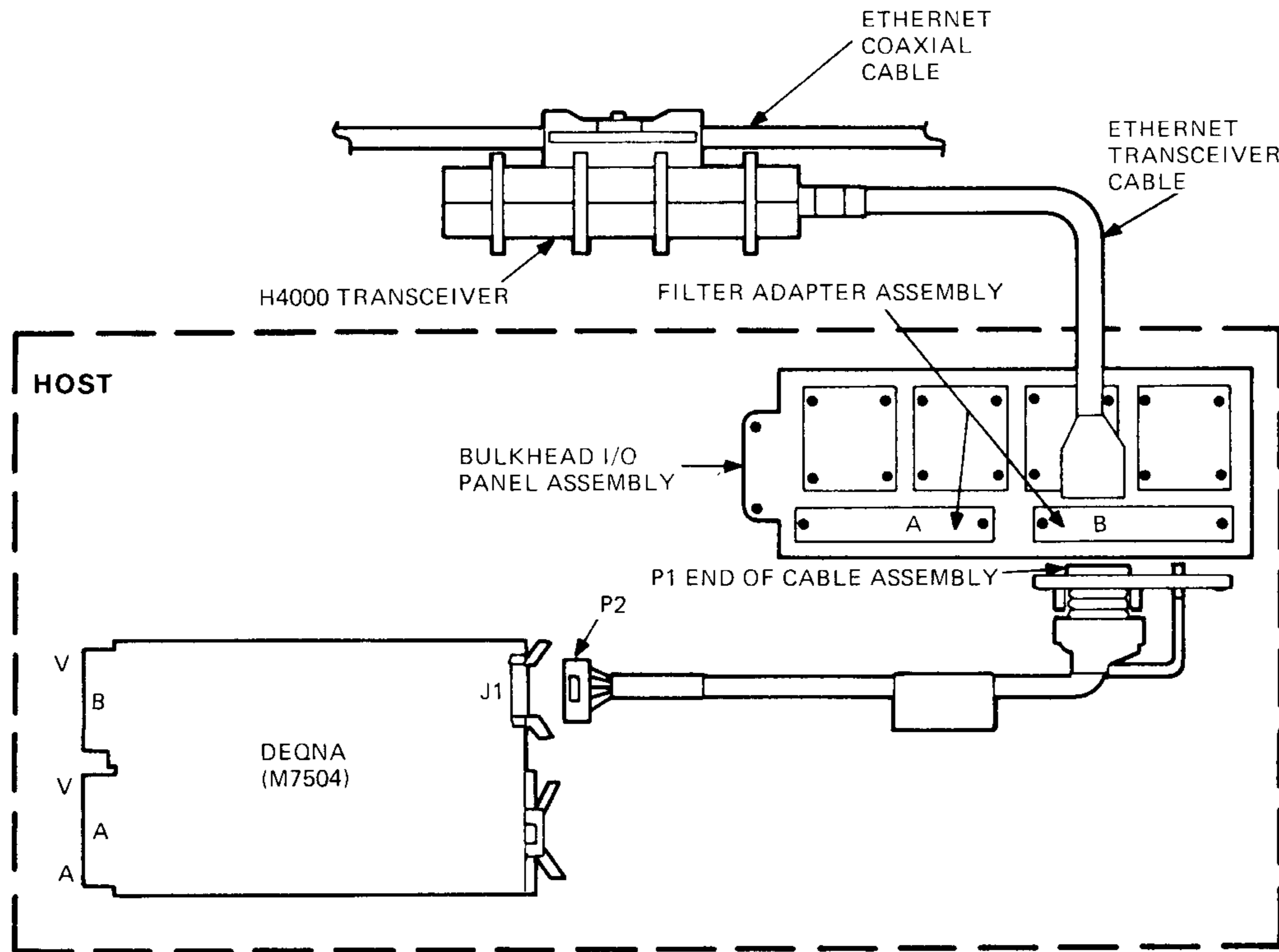
Figure 1-4 DEQNA to ETHERNET Connection
